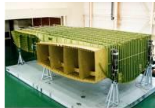
Wing Center Section
